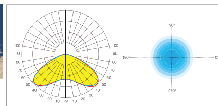
120° Application: Symmetric light distribution for square, park, highbay lighting.
