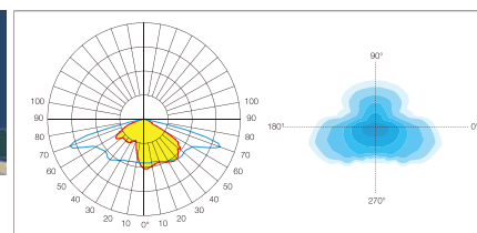
T3A 80 x 150° Application: Asymmetric light distribution for Residential street.
