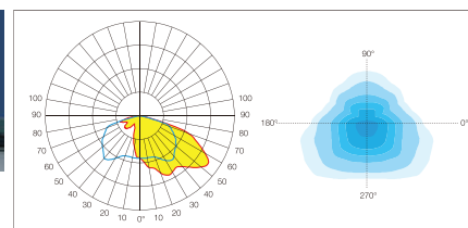
T4A 50 x 150° Application: Asymmetric light distribution for wide area.
